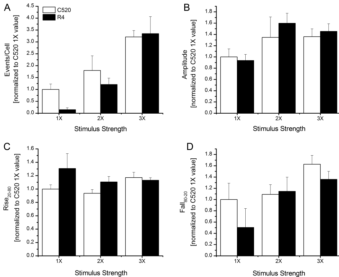
Fig. 4. Head-to-head comparison of C520 versus R4 for detecting and measuring \text{Ca}^{2+} puffs evoked by varying amounts of photoreleased \text{i-IP}_3 . UV photolysis flashes were of constant intensity and durations of 25 ms (1 \times ), 50 ms (2 \times ) and 75 ms (3 \times ). Bar graphs show mean numbers of events evoked per cell per second (A), mean puff amplitudes (B), mean puff rise time (C) and mean puff fall time (D) of local \text{Ca}^{2+} signals detected by C520 (open bars) and R4 (filled bars) in response to the different stimuli. All data are shown normalized relative to the mean values obtained using C520 with the 1 \times flash duration. A range of 98–99 (1 \times ), 172–178 (2 \times ), and 271–287 (3 \times ) local events for C520 and 7–8 (1 \times ), 115–117 (2 \times ), and 415–428 (3 \times ) for R4 were analyzed from 3 to 6 experiments for each stimulus strength. Values were normalized to the mean C520 1X value for each parameter and are presented as mean \pm 1 SEM.
