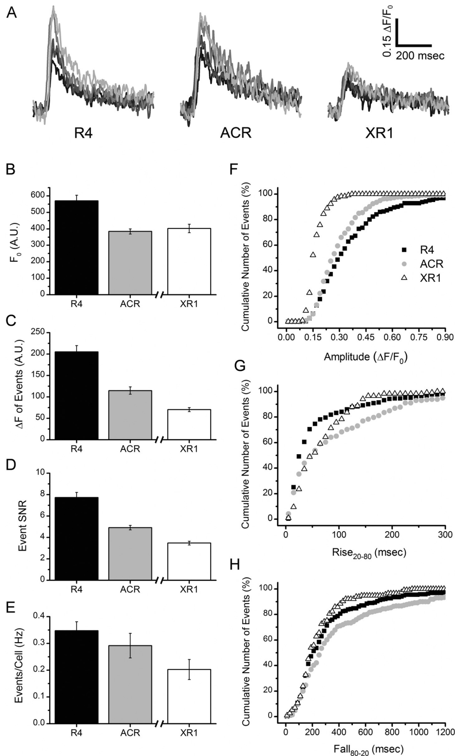
Fig. 3. Analysis of local \text{Ca}^{2+} puffs imaged by red-emitting fluorescent \text{Ca}^{2+} indicator dyes; Rhod-4 (R4), Asante Calcium Red (ACR) and X-Rhod-1 (XR1). Each indicator was individually evaluated under identical conditions in SH-SY5Y cells, with the exception that R4 and ACR were excited with a 532 nm laser whereas XR1 was excited with a 561 nm laser. For this reason, measurements of resting fluorescence of XR1 ( F_0 , panel B) cannot be directly compared with the other two indicators. Otherwise, results are presented in the same way as Fig. 2. Data in (B–E) are expressed as the mean \pm SEM from 8 trials for each indicator. Total numbers of events in cumulative probability graphs (F–H) are at least 215 (R4), 211 (ACR), and 113 (XR1).
