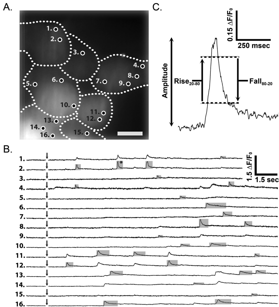
Fig. 1. Experimental protocol for imaging local \text{Ca}^{2+} puffs evoked in SH-SY5Y cells by photo-released \text{i-IP}_3 . (A) Resting fluorescence of several cells (outlined) which were loaded with Cal-520 and caged \text{i-IP}_3 . Circles mark sites at which puffs were observed following photo-released \text{i-IP}_3 . Scale bar = 10 \mu\text{m} . (B) Traces depict simultaneous measurement of Cal-520 fluorescence over time ( \Delta F/F_0 ) from the numbered sites in panel (A). A flash of UV light (75 ms duration) was delivered uniformly throughout the imaging field when marked by the arrows. Traces are scaled as the change in fluorescence ( \Delta F ) divided by the resting fluorescence ( F_0 ) at that site before stimulation, and were derived using an automated algorithm to identify the site of origin of each event (marked by grey boxes). (C) A single \text{Ca}^{2+} puff (identified by an asterisk in B) shown on expanded scales to illustrate measurements of amplitude and rise and fall times.
