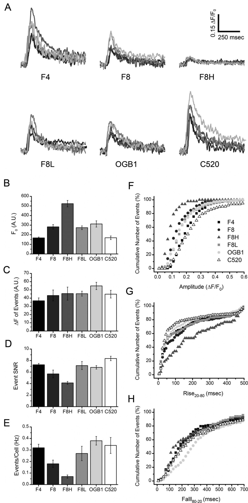
Fig. 2. Analysis of local \text{Ca}^{2+} puffs imaged by green-emitting fluorescent \text{Ca}^{2+} indicator dyes. (A) Representative traces showing \text{Ca}^{2+} puffs recorded using different indicators; Fluo-4 (F4), Fluo-8 (F8), Fluo-8 high affinity (F8H), Fluo-8 low affinity (F8L), Oregon Green BAPTA-1 (OGB1), and Cal-520 (C520). Fluorescence signals are scaled as \Delta F/F_0 , and superimposed traces are aligned to their peak time and depicted in different shades of grey for clarity. All events were evoked by photo-released i-IP 3 under identical stimulus and recording conditions. Bar graphs (B and C) show measurements for each indicator of; (B) background subtracted resting cell fluorescence ( F_0 ) in arbitrary camera units (A.U.), (C) peak amplitudes of puffs ( \Delta F ), (D) signal-to-noise ratio (SNR) of puffs, and (E) the number of puffs detected per cell per second. Mean values were calculated for all cells and puffs within a given imaging field (trial), and bars show mean \pm SEM from 6 trials for each indicator (F–G). Cumulative probability plots showing, for each indicator (depicted by different symbols), the percentage of all detected events as functions of; (F) puff amplitude ( \Delta F/F_0 ), (G) puff rise time (rise 20–80 ), and (H) fall time (fall 80–20 ). Total numbers of events analyzed for each parameter were at least 145 (Fluo-4), 100 (Fluo-8), 39 (Fluo-8H), 115 (Fluo-8L), 239 (OGB1), and 150 (Cal-520); in some instances signals were too small to obtain reliable measurements of fall time.
