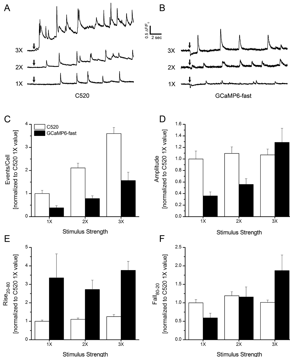
Fig. 6. Head-to-head comparison of Cal-520 versus GCaMP6-fast for detecting and measuring \text{Ca}^{2+} puffs evoked by varying amounts of photo-released \text{i-IP}_3 . (A and B) Representative traces showing local \text{Ca}^{2+} signals evoked by UV photolysis flashes of constant intensity and varying durations of 25 ms (1 \times ), 50 ms (2 \times ) and 75 ms (3 \times ) recorded, respectively, using Cal-520 and GCaMP6-fast. Transient downward deflections in the GCaMP traces likely reflect photobleaching by the UV flashes. (C–F) Bar graphs show mean numbers of events evoked per cell per second (C), mean puff amplitudes (D), mean puff rise time (E) and mean puff fall time (F) of local \text{Ca}^{2+} signals detected by Cal-520 (open bars) and GCaMP6-fast (filled bars) in response to the different stimuli. All data are shown normalized relative to the mean values obtained using Cal-520 with the 1 \times flash duration and are presented as mean \pm SEM. Measurements with Cal-520 were made from at least 175 (1 \times flash), 327 (2 \times ), and 258 (3 \times ) local events; and for GCaMP6-fast from at least 23 (1 \times ), 62 (2 \times ), and 105 (3 \times ) events.
